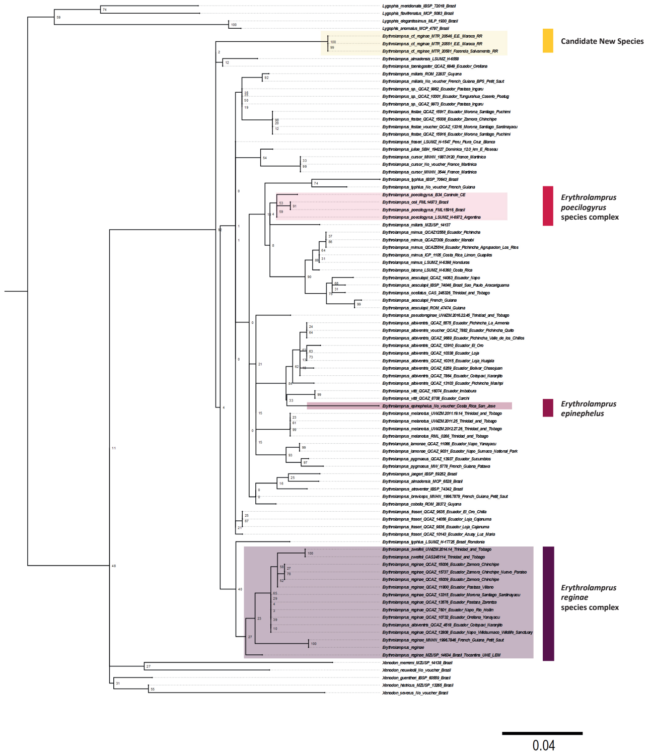
Supplementary File 2. Phylogenetic analysis as per maximum likelihood, branches equal to genetic distance.
